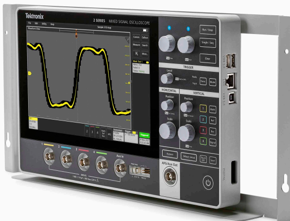
Rackmount kit
