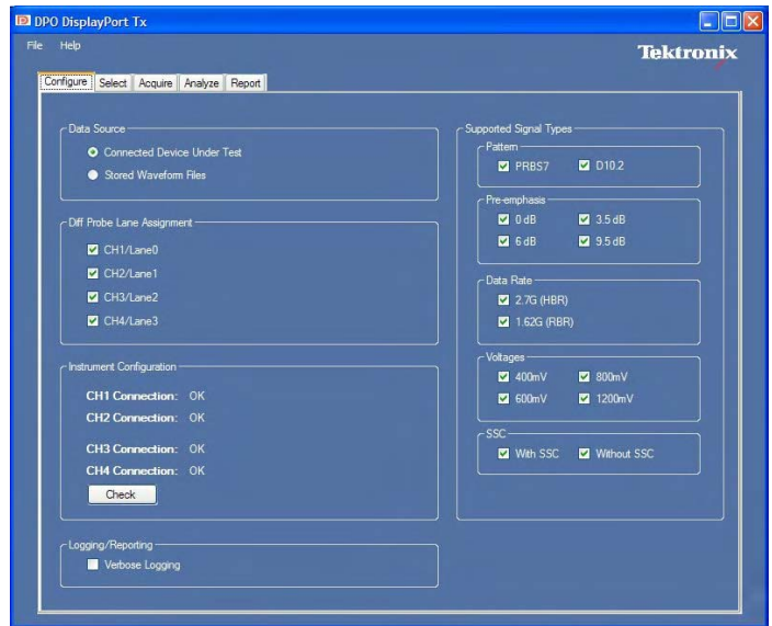
DisplayPort Compliance Test Solution (Option DSPT) – Supports DisplayPort Compliance Test Standard (CTS) source test with four-line simultaneous testing using the Tektronix P7300SMA Series probes and DisplayPort software. Detailed test reports with waveform plots, pass/fail results, and margin analysis are included.
