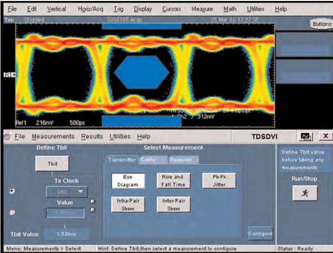
DVI Compliance Test Solution (Option DVI) – Obtain quick and dependable results with the DVI compliance test software. Automated testing based on pass/fail detection dramatically enhances productivity.
