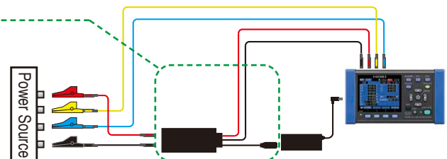
Obtains power from the measurement lines
