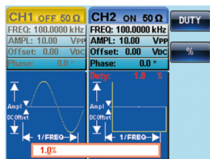
1% Duty Cycle of Square Wave
