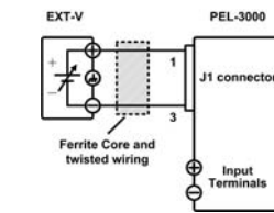
External Voltage Connection
