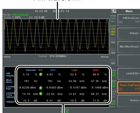
AM modulation measurements
