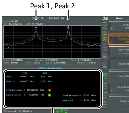
2FSK measurement
