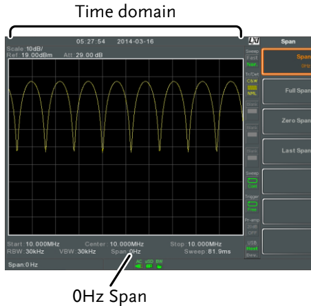
0Hz Span Example: Amplitude modulation
