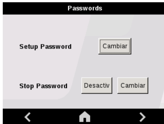
Figura 63: Password.
