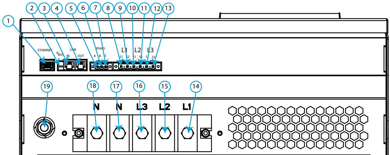
Figura 11:Bornes SVGm-xxx-100M.
