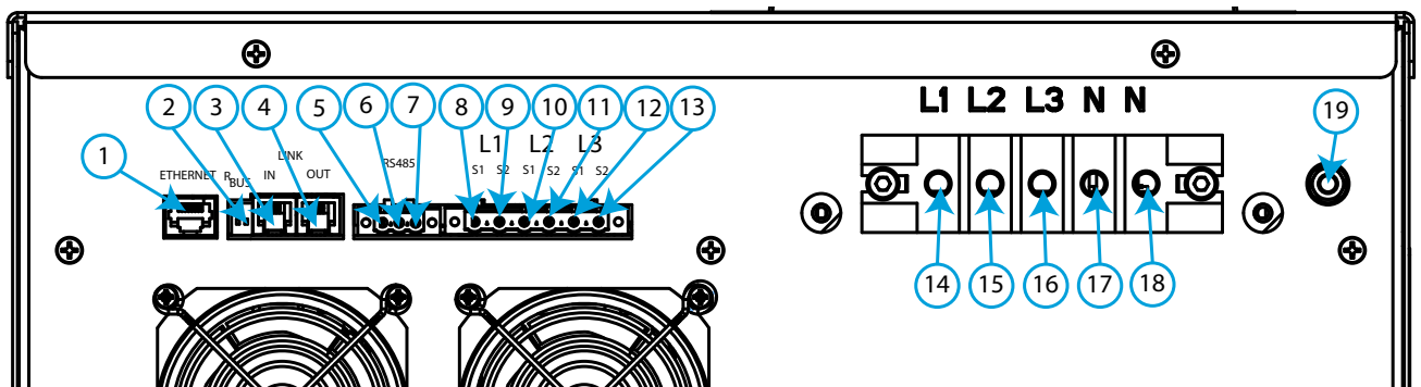
Figura 10:Bornes SVGm-xxx-030M y SVGm-xxx-060M.
